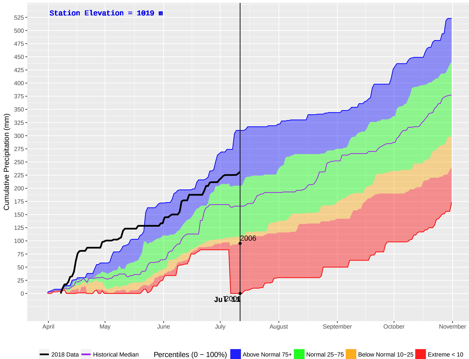
POWDER CREEK (380) : Historical (2001–2016) and Current (2018) Noon Cumulative Precipitation
