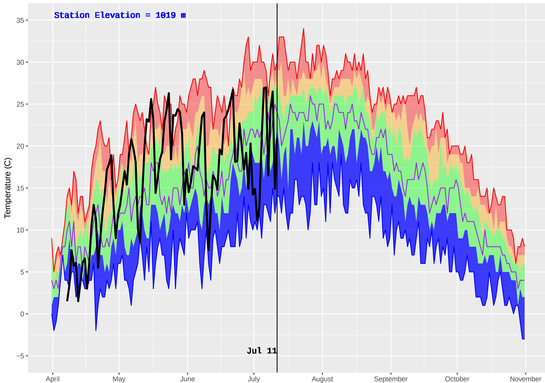
POWDER CREEK (380) : Historical (2001–2016) and Current (2018) Noon Temperature
