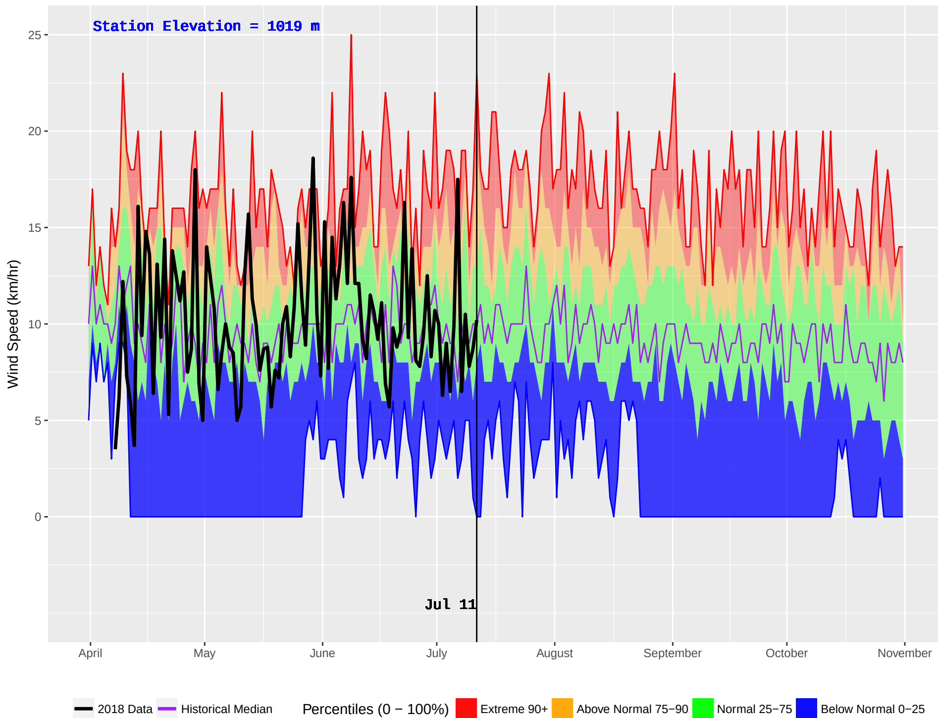
POWDER CREEK (380) : Historical (2001–2016) and Current (2018) Noon Wind Speed
