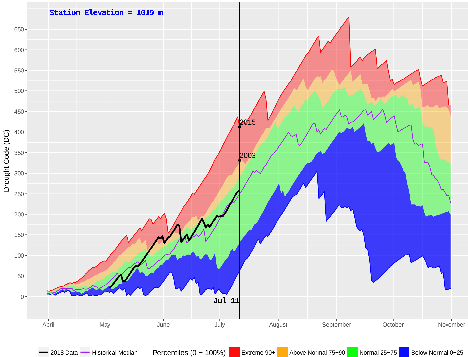
POWDER CREEK (380) : Historical (2001–2016) and Current (2018) Noon Drought Code (DC)
